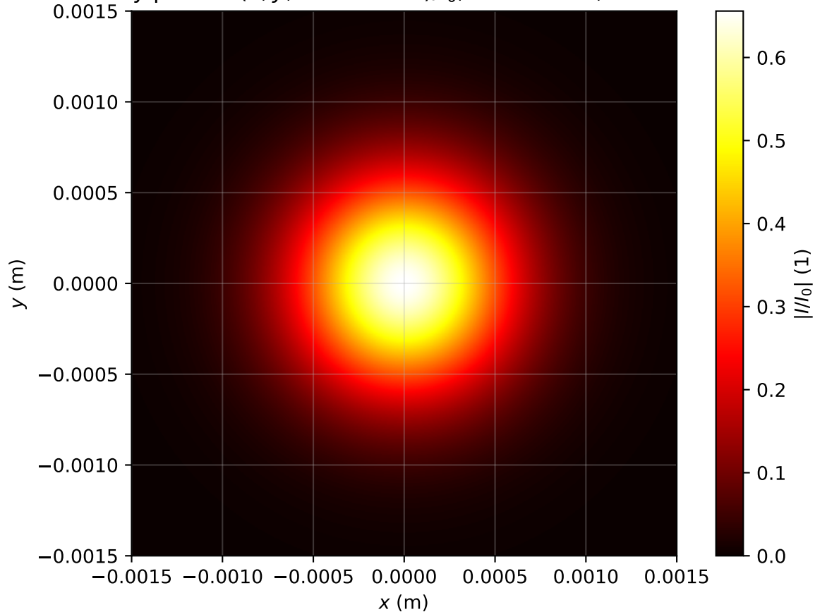
Intensity profile I(x, y, z = 1.990m)/I_0 , \text{Pin}=0.3\text{Pcr} , artificial time
